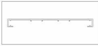
26X341 Silent mouthpiece wall thickness: 3.8 mm Applicable wall thickness: 298mm-319mm
