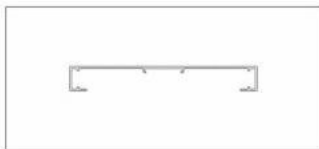
24.8X230 Silent mouthpiece wall thickness: 2.3 mm Applicable wall thickness: 188mm-207mm
