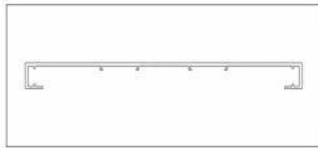
26X320 silent mouthpiece wall thickness: 3.8 mm Wall thickness: 278mm-297mm
